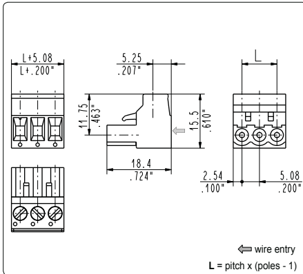
CIF_005 side stackable female
