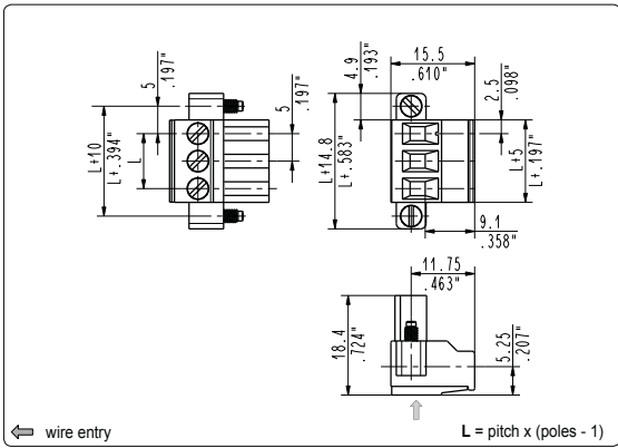
CIF_0V1 locking screw flanges, female
