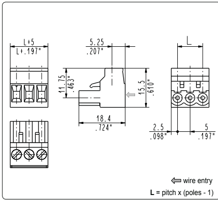
CIF_001 side stackable female
