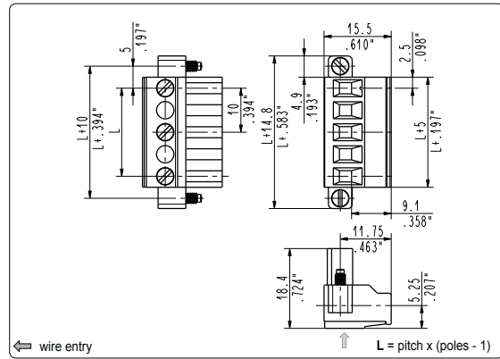
CIF_0V2 locking screw flanges, female
