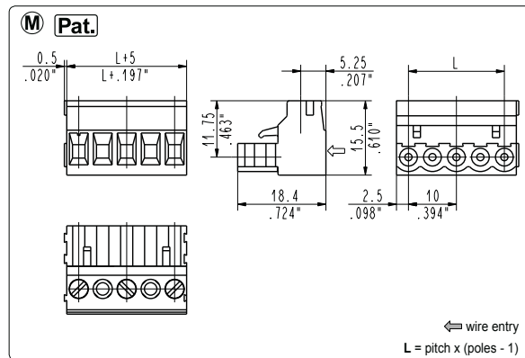
CIF_OM2 modular female
