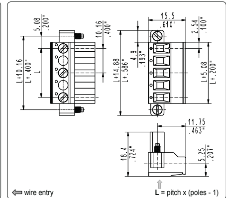
CIF_0V6 locking screw flanges, female
