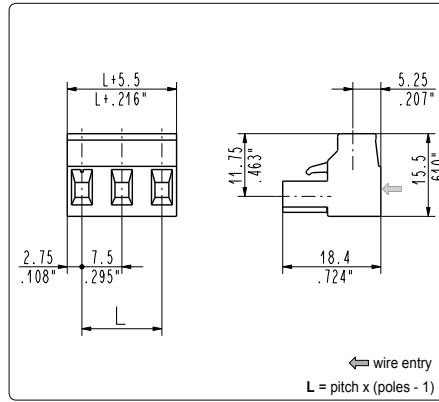
CIF_003 side stackable female
