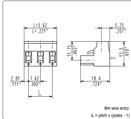
CIF_007 side stackable female
