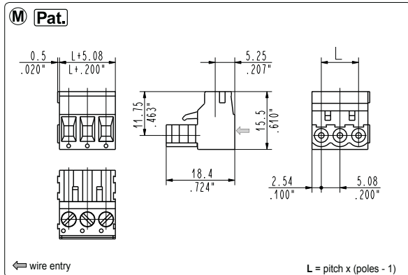
CIF_OM5 modular female
