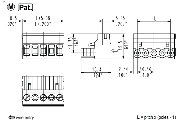
CIF_OM6 modular female
