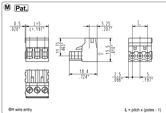
CIF_OM1 modular female
